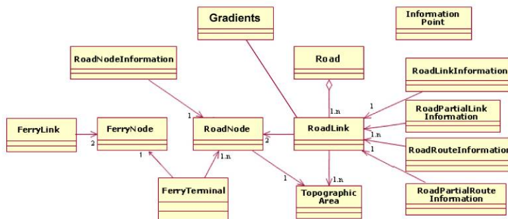
Figure 1: ITN Layer data model including gradient information.
