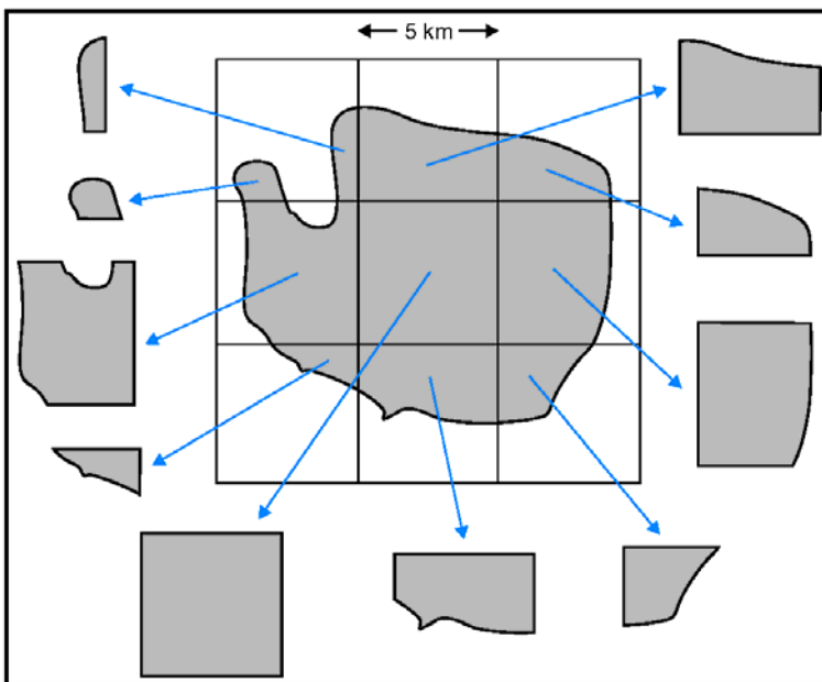
Figure 21: chunking
